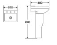
DR-326P Basin With Pedestal 610x480x840mm Fixing To Wall With Back
