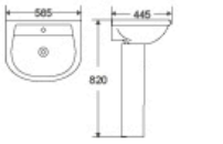
DR-342P Basin With Pedestal 565x445x820mm Fixing To Wall With Back
