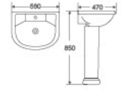
DR-344P Basin With Pedestal 560x470x850mm Fixing To Wall With Back
