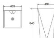
DR-307 Basin With Pedestal 460x460x840mm Fixing To Wall With Back
