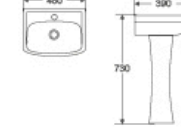
DR-301P Pedestal Basin 480x390x730mm Fixing To Wall With Back
