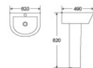
DR-312P Basin With Pedestal 620x490x820mm Fixing To Wall With Back
