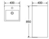
DR-309 Pedestal Basin 400x400x850mm Fixing To Wall With Back
