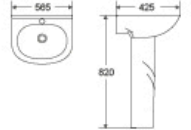
DR-318P Pedestal Basin 565x425x820mm Fixing To Wall With Back
