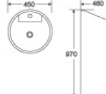
DR-305 Pedestal Basin 450x460x970mm Fixing To Wall With Back
