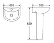
DR-316P Basin With Pedestal 660x505x820mm Fixing To Wall With Back
