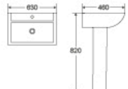
DR-306P Pedestal Basin 630x460x820mm Fixing To Wall With Back
