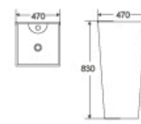
DR-303 Pedestal Basin 470x470x830mm Fixing To Wall With Back
