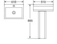
DR-328P Basin With Pedestal 615x510x865mm Fixing To Wall With Back
