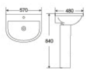
DR-332P Basin With Pedestal 570x480x840mm Fixing To Wall With Back
