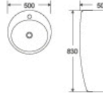
DR-311 Basin With Pedestal 500x500x830mm Fixing To Wall With Back
