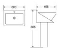
DR-329P Basin With Pedestal 600x455x805mm Fixing To Wall With Back
