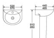
DR-321P Basin With Pedestal 520x440x810mm 570x465x850mm Fixing To Wall With Back
