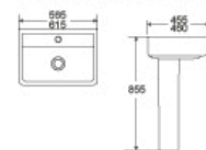
DR-350P Basin With Pedestal 565x455x855mm 615x460x855mm Fixing To Wall With Back
