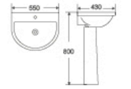
DR-340P Basin With Pedestal 550x430x800mm Fixing To Wall With Back
