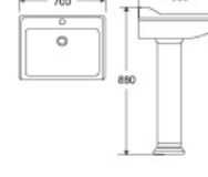
DR-339P Basin With Pedestal 700x550x880mm Fixing To Wall With Back
