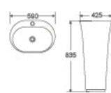
DR-315 Basin With Pedestal 590x425x835mm Fixing To Wall With Back
