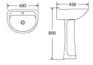
DR-322P Pedestal Basin 490x430x800mm Fixing To Wall With Back
