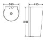
DR-319 Pedestal Basin 540x480x810mm Fixing To Wall With Back
