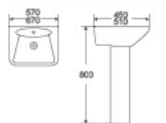
DR-334P Basin With Pedestal 570x450x800mm 670x510x800mm Fixing To Wall With Back
