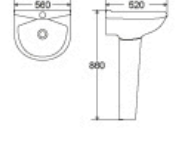
DR-317P Basin With Pedestal 560x520x860mm Fixing To Wall With Back
