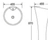
DR-313 Pedestal Basin 455x455x870mm Fixing To Wall With Back
