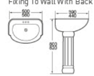
DR-347P Basin With Pedestal 500x390x800mm 560x440x820mm Fixing To Wall With Back
