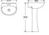
DR-345P Basin With Pedestal 575x450x810mm Fixing To Wall With Back
