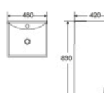
DR-314 Basin With Pedestal 480x420x830mm Fixing To Wall With Back
