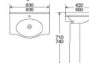
DR-305P Basin With Pedestal 600x420x710mm 800x500x740mm Fixing To Wall With Back
