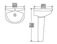
DR-336P Basin With Pedestal 570x480x790mm 665x510x890mm Fixing To Wall With Back
