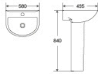
DR-315P Basin With Pedestal 560x435x840mm Fixing To Wall With Back
