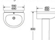
DR-310P Pedestal Basin 560x450x800mm 680x500x800mm Fixing To Wall With Back
