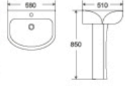
DR-303P Pedestal Basin 580x510x850mm Fixing To Wall With Back
