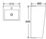
DR-304 Basin With Pedestal 510x450x845mm Fixing To Wall With Back
