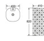
DR-316 Basin With Pedestal 420x410x820mm Fixing To Wall With Back
