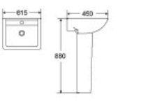
DR-338P Basin With Pedestal 615x450x880mm Fixing To Wall With Back
