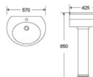
DR-331P Basin With Pedestal 570x425x850mm Fixing To Wall With Back
