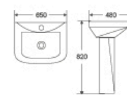
DR-307P Basin With Pedestal 650x480x820mm Fixing To Wall With Back
