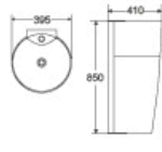
DR-302 Basin With Pedestal 410x395x850mm Fixing To Wall With Back
