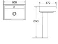
DR-325P Basin With Pedestal 600x470x850mm Fixing To Wall With Back
