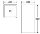
DR-312 Pedestal Basin 400x400x850mm Fixing To Wall With Back
