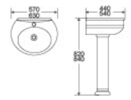
DR-337P Basin With Pedestal 570x440x820mm 630x540x840mm Fixing To Wall With Back
