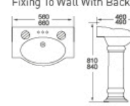
DR-346P Basin With Pedestal 560x460x810mm 660x490x840mm Fixing To Wall With Back
