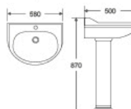
DR-330P Basin With Pedestal 580x500x870mm Fixing To Wall With Back
