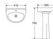
DR-311P Pedestal Basin 410x350x750mm Fixing To Wall With Back
