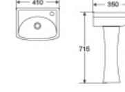
DR-302P Pedestal Basin 410x350x715mm Fixing To Wall With Back
