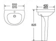
DR-335P Basin With Pedestal 510x400x825mm 570x455x825mm Fixing To Wall With Back
