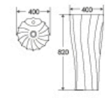
DR-317 Pedestal Basin 400x400x820mm Fixing To Wall With Back
